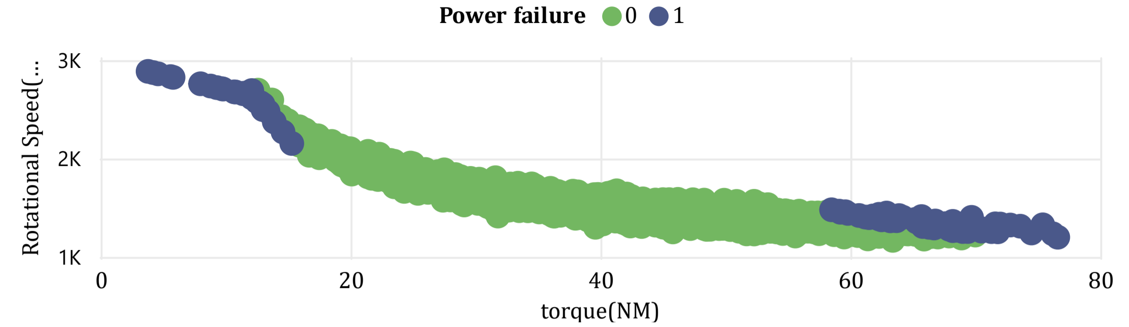
Torque vs Rotational Speed by Power Failure
