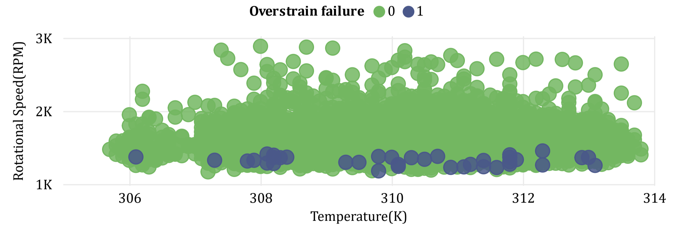
Temperature vs RPM — Overstrain Failure
